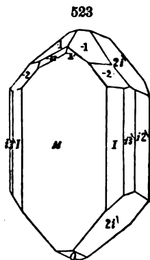
Norwich, Mass.
